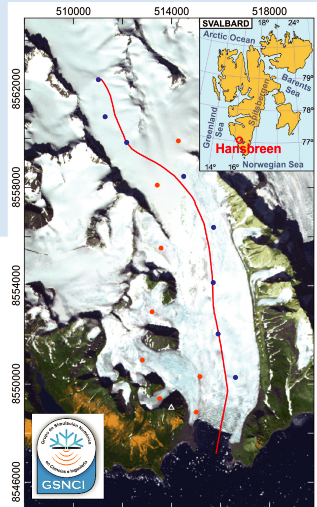
Fig. 1 Hansbreen glacier with location of velocity and mass balance stakes and the modelled central flowline.
