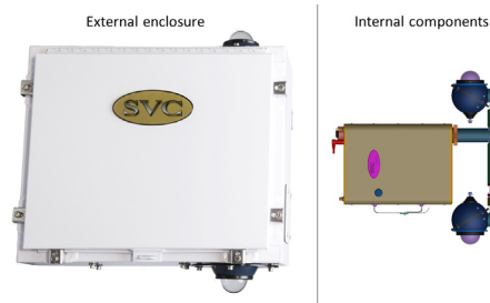
Fig. 2 View of the SVC instrument (left) and its internal components (right) where it is connected to the optical tube and the two integrating spheres.
