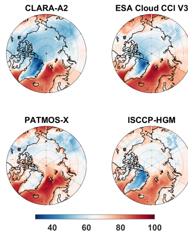
Fig. 2 Comparison of climatological mean cloud fraction in four CDRs (1982-2016).
