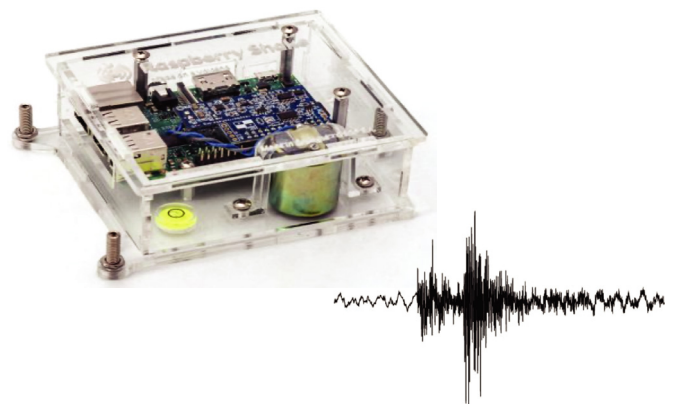
Fig. 2 Upper: photo of the Raspberrysshake seismometer, Lower: a seismogram showing the recording of a magnitude 2.0 earthquake located 122 km South-West of Akunnaaq, May 21st 2018.
