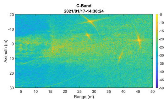
Fig. 2 Examples of SodSAR imagery of backscatter (in dB) of a forested site. Imaging direction from left to right. Corner reflectors used for calibration appear as bright objects in the images.
