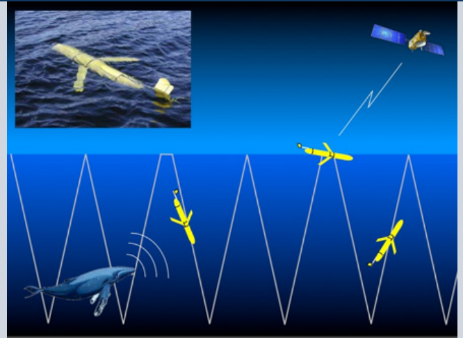
Fig. 1 Glider operational mode.
